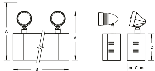
EF150 Cabinet information
